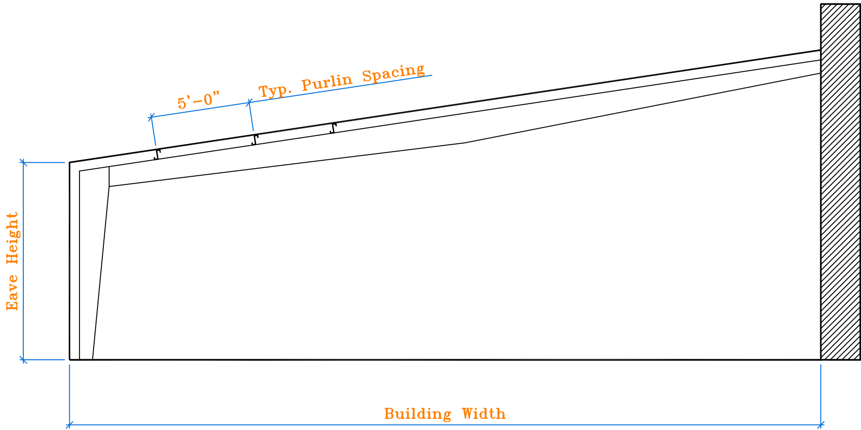
LEAN-TO FRAME
