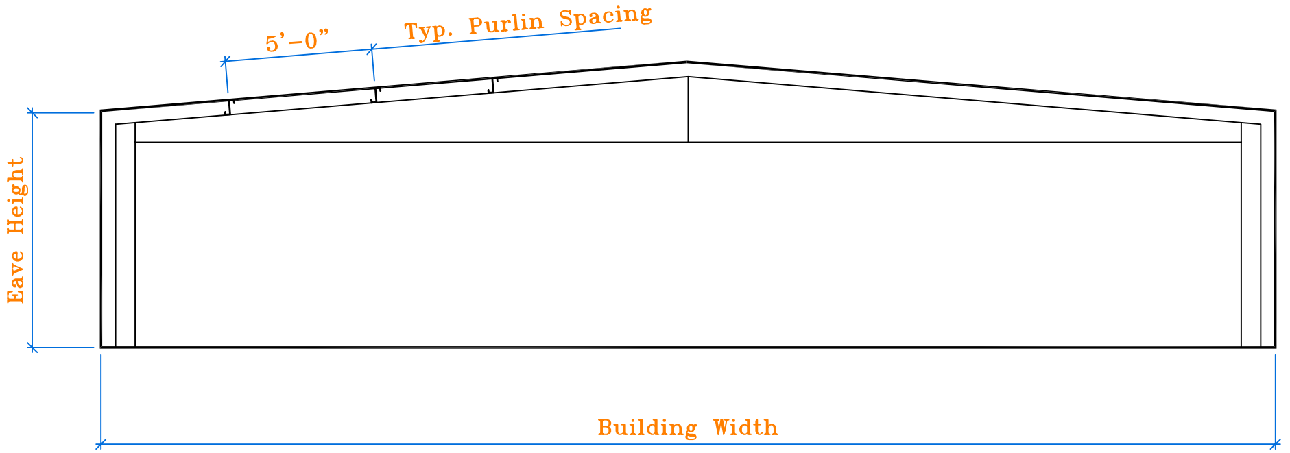
TAPERED BEAM FRAME
